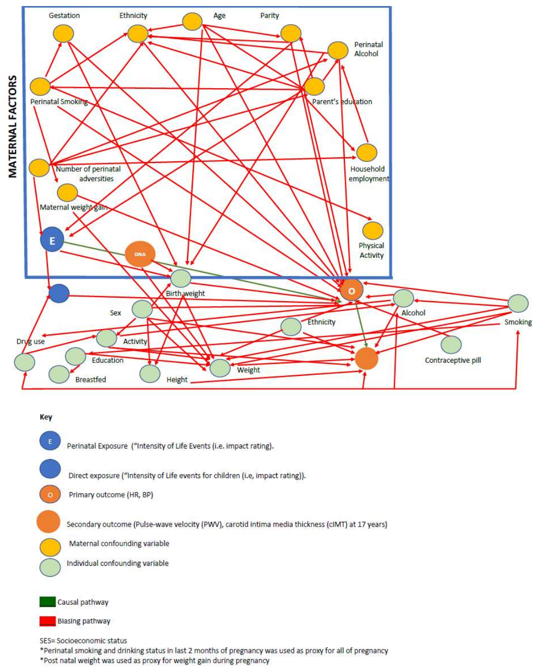
Supplementary Figure S2: Directed Acyclic Graph at seventeen years of age
